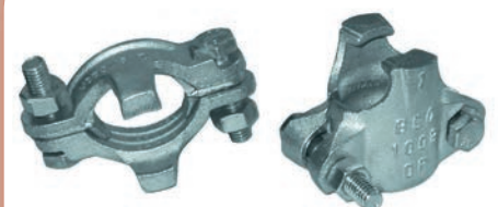
Hercules con griffe Hercules hose clamps with safety claws
